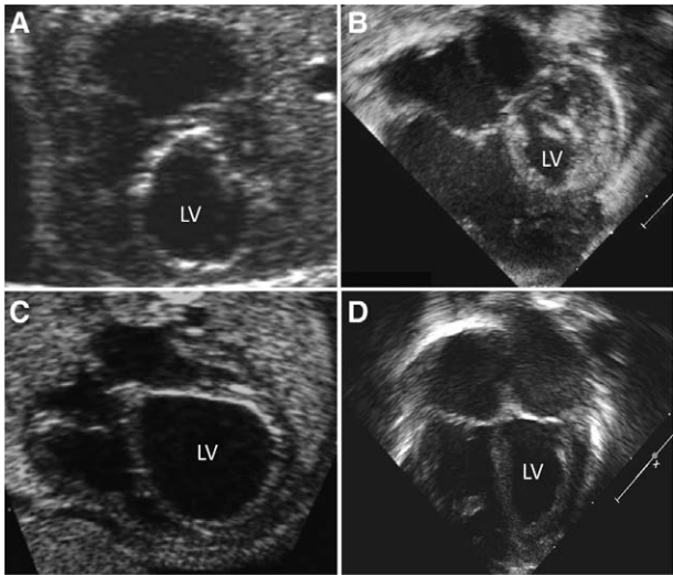
Figure 3. Preintervention fetal and neonatal echocardiograms of a patient who underwent technically unsuccessful fetal aortic valvuloplasty (FAV) and was managed with a univentricular strategy (A and B), and a patient who underwent technically successful FAV and was managed as biventricular postnatally (C and D). LV indicates left ventricle.
